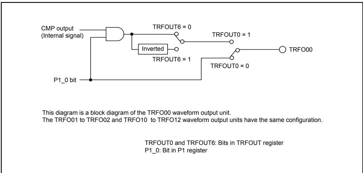
Figure 17.47 Block Diagram of CMP Waveform Output Unit
