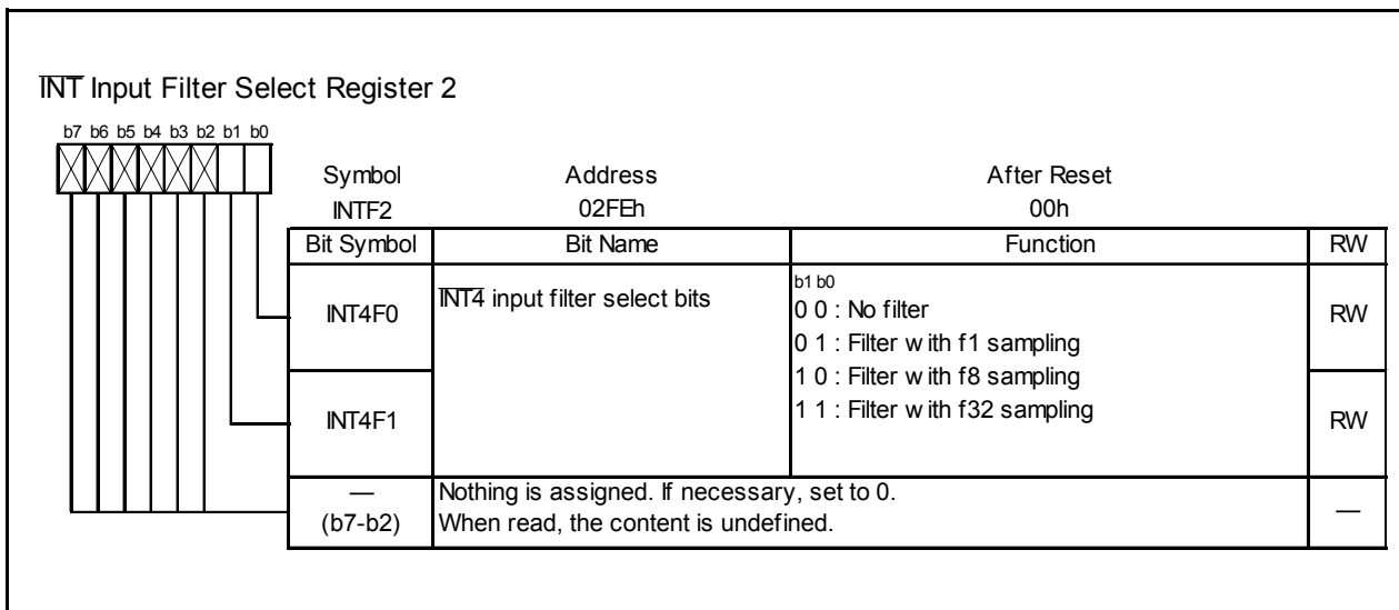
Figure 13.14 INTF2 Register
